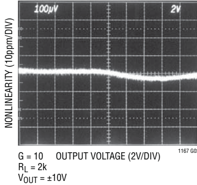
Gain Nonlinearity, G = 10
