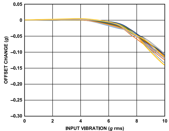
Figure 71. VRE, Y-Axis Offset from +1 g, ±10 g Range, Y-Axis Orientation = +1 g
