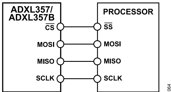
Figure 91. 4-Wire SPI Connection
