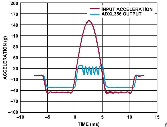
Figure 85. ADXL356 Overrange Behavior for \pm 20 g Range Setting
