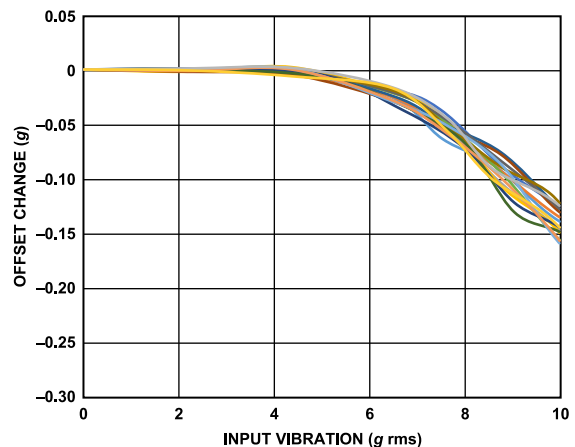
Figure 72. VRE, Z-Axis Offset from +1 g, ±10 g Range, Z-Axis Orientation = +1 g
