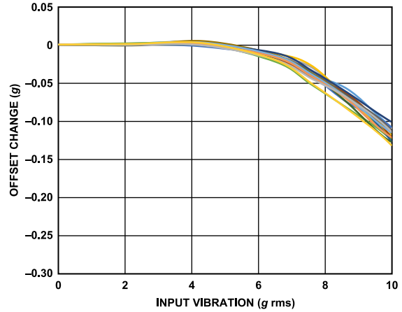
Figure 70. VRE, X-Axis Offset from +1 g, ±10 g Range, X-Axis Orientation = +1 g
