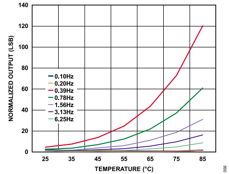
Figure 44. Typical X-Axis Output vs. Temperature at Lower Data Rates, Normalized to 100 Hz Output Data Rate, V_S = 2.5\text{ V}
