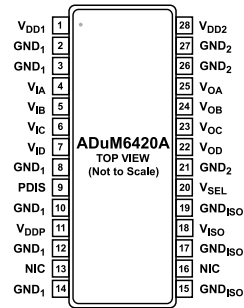
Figure 3. ADuM6420A Pin Configuration
