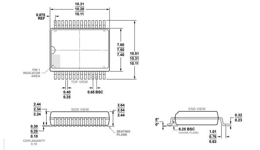
Figure 28. 28-Lead Standard Small Outline, Wide Body, with Finer Pitch [SOIC_W_FP] (RN-28-1) Dimensions shown in millimeters
