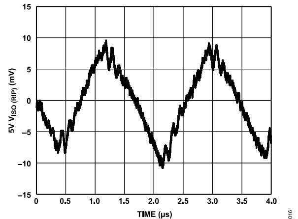
Figure 18. Output Voltage Ripple at 90% Load, V_{ISO} = 5 V
