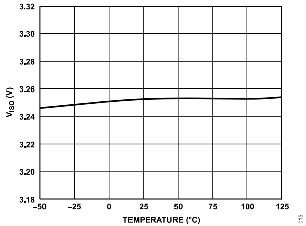
Figure 17. V_{ISO} vs. Temperature, Input = 3.3 V, V_{ISO} = 3.3 V
