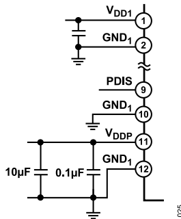
Figure 23. V_{DD1} and V_{DDP} Bias and Bypass Components
