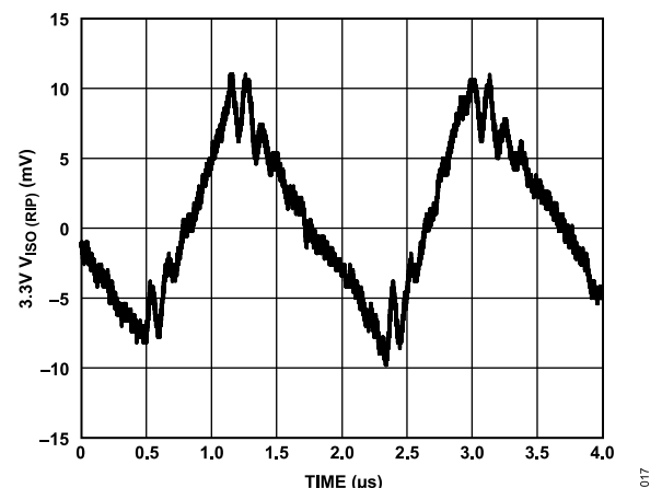
Figure 19. Output Voltage Ripple at 90% Load, V_{ISO} = 3.3 V
