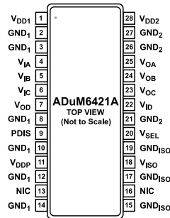
Figure 4. ADuM6421A Pin Configuration
