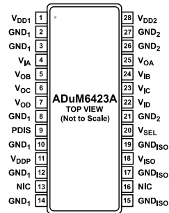
Figure 6. ADuM6423A Pin Configuration
