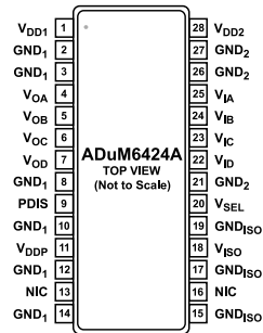
Figure 7. ADuM6424A Pin Configuration
