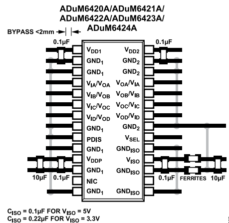
Figure 25. Recommended PCB Layout
