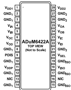
Figure 5. ADuM6422A Pin Configuration
