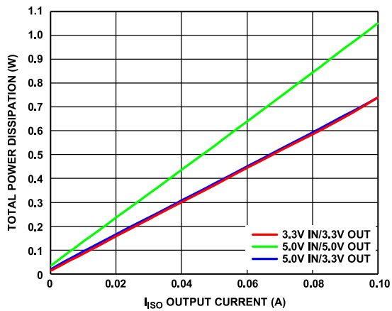
Figure 10. Total Power Dissipation vs. I_{ISO} Output Current in Supported Power Configurations
