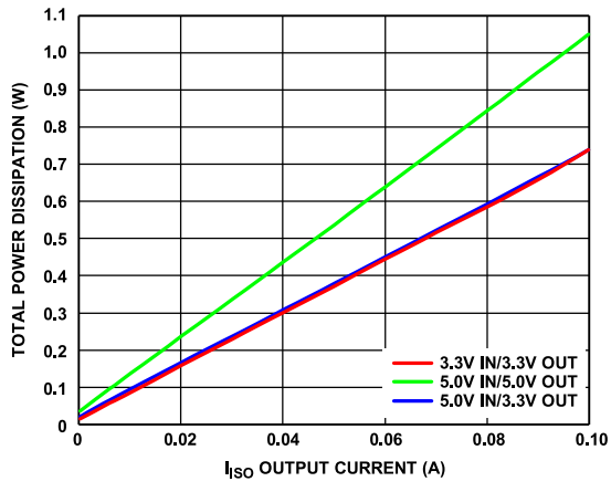
Figure 10. Total Power Dissipation vs. I_{ISO} Output Current in Supported Power Configurations
