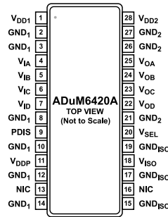
Figure 3. ADuM6420A Pin Configuration
