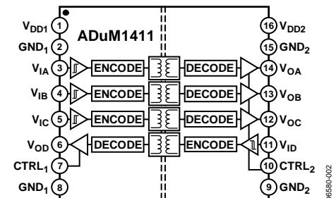
Figure 2. ADuM1411
