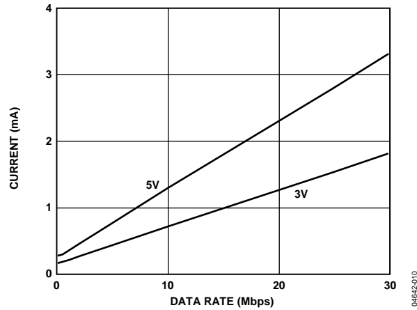
Figure 10. Typical ADuM1201 V_{DD2} Supply Current vs. Data Rate for 5 V and 3 V Operation
