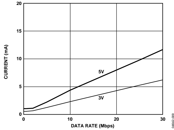
Figure 9. Typical ADuM1201 V_{DD1} Supply Current vs. Data Rate for 5 V and 3 V Operation
