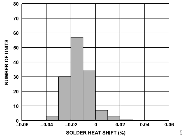
Figure 33. ADR4550 Solder Heat Resistance Shift (3 x Reflow)
