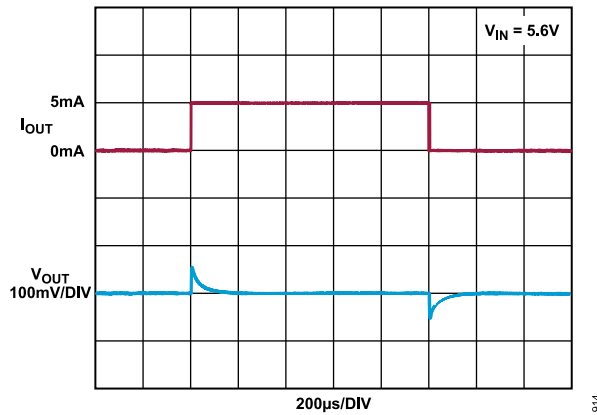
Figure 78. ADR4550 A, B, and C Grades Load Transient Response (Sinking)
