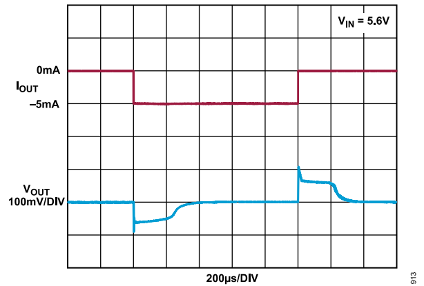
Figure 81. ADR4550 A, B, and C Grades Load Transient Response (Sourcing)
