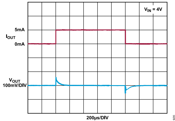
Figure 31. ADR4550 A, B, and C Grades Load Transient Response (Sinking)
