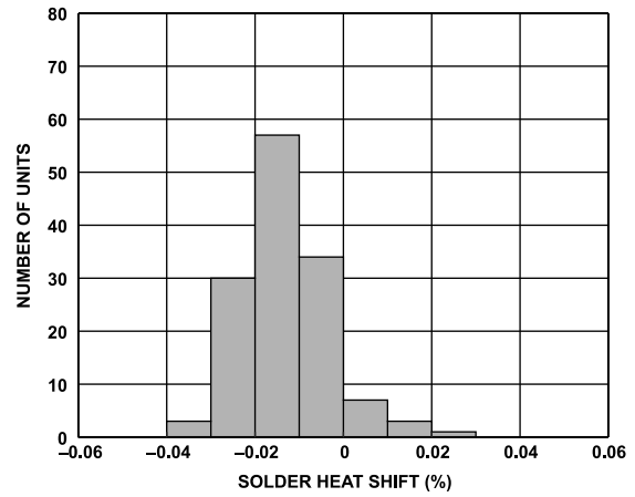
Figure 80. ADR4550 Solder Heat Resistance Shift (3 × Reflow)
