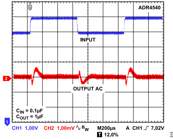
Figure 77. ADR4550 Line Transient Response
