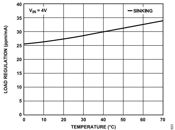
Figure 35. ADR4550 D Grade Load Regulation vs. Temperature (Sinking)
