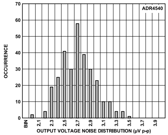
Figure 74. ADR4550 Output Voltage Noise (Maximum Amplitude from 0.1 Hz to 10 Hz)
