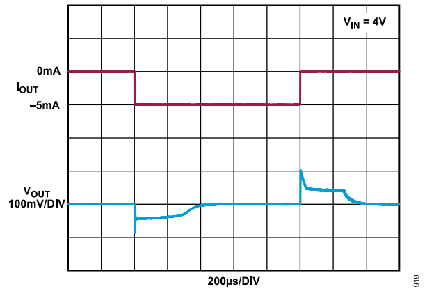
Figure 34. ADR4550 A, B, and C Grades Load Transient Response (Sourcing)
