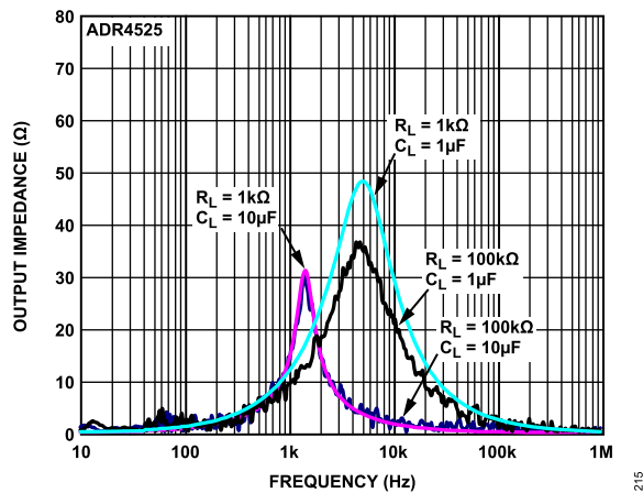
Figure 32. ADR4550 Output Impedance vs. Frequency
