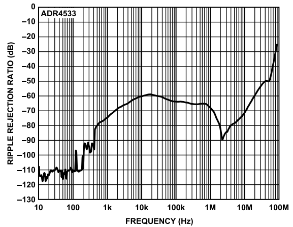
Figure 61. ADR4533 Ripple Rejection Ratio vs. Frequency
