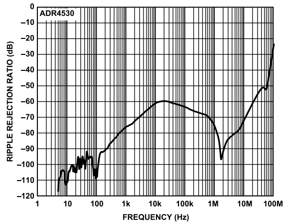
Figure 48. ADR4530 Ripple Rejection Ratio vs. Frequency
