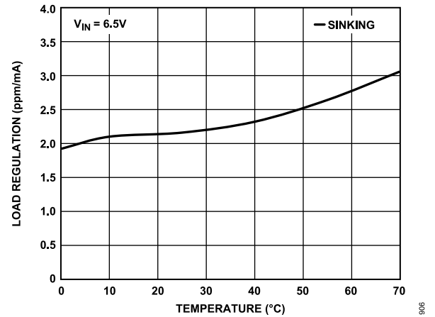
Figure 103. ADR4550 D Grade Load Regulation (Sinking)
