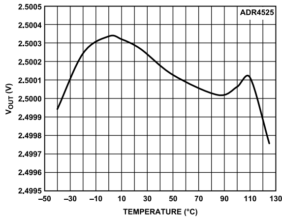
Figure 18. ADR4525 B Grade Output Voltage vs. Temperature
