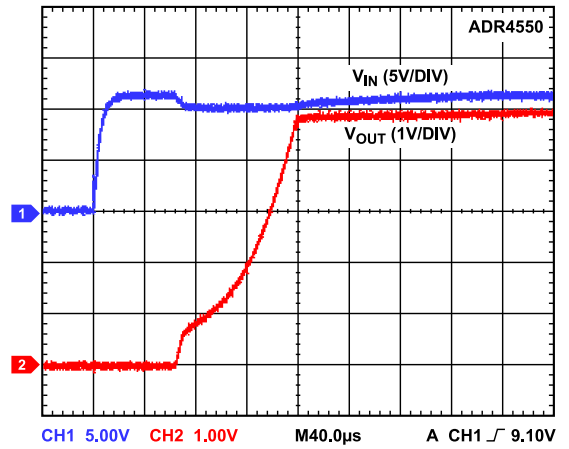
Figure 89. ADR4550 Output Voltage Start-Up Response
