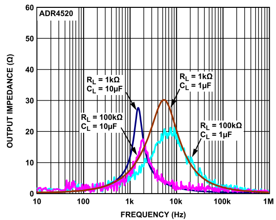
Figure 16. ADR4520 Output Impedance vs. Frequency
