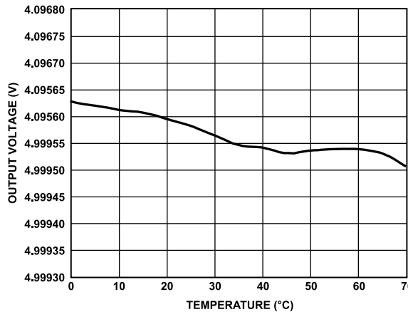
Figure 88. ADR4550 D Grade Output Voltage vs. Temperature
