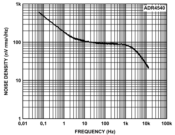
Figure 75. ADR4540 Output Noise Spectral Density
