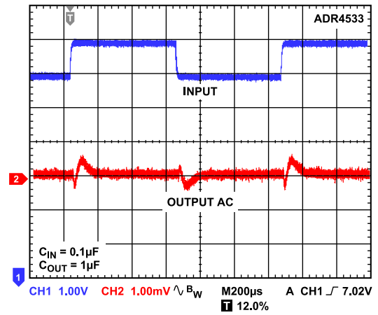
Figure 62. ADR4530 Line Transient Response
