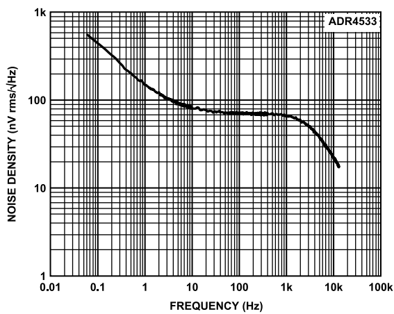
Figure 60. ADR4530 Output Noise Spectral Density
