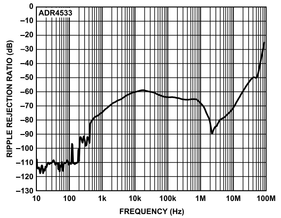
Figure 61. ADR4530 Ripple Rejection Ratio vs. Frequency
