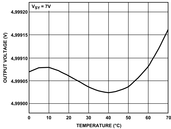
Figure 87. ADR4550 C Grade Output Voltage vs. Temperature
