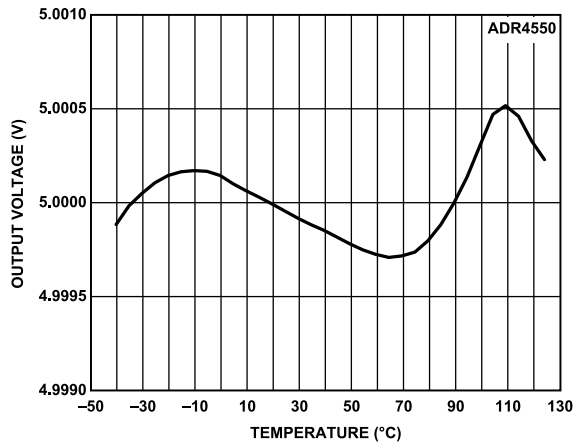
Figure 86. ADR4550 B Grade Output Voltage vs. Temperature
