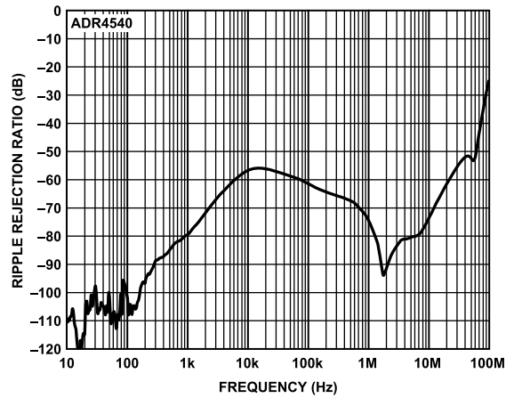
Figure 76. ADR4540 Ripple Rejection Ratio vs. Frequency
