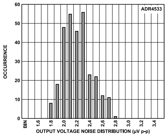
Figure 59. ADR4530 Output Voltage Noise (Maximum Amplitude from 0.1 Hz to 10 Hz)
