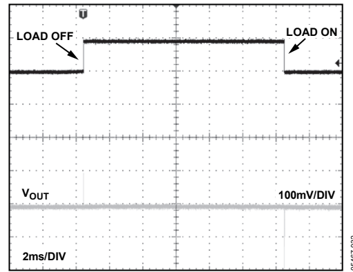
Figure 30. ADR366 Load Transient Response
