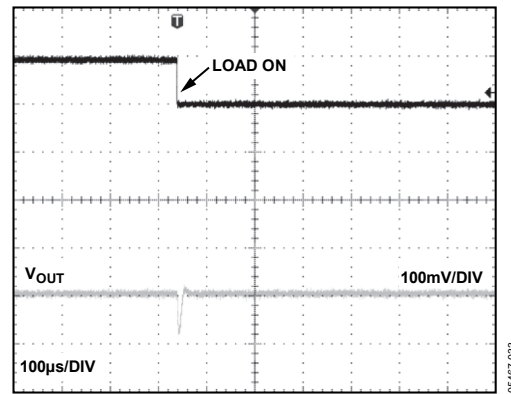
Figure 31. ADR366 Load Transient Response with 0.1 \mu F Output Capacitor
