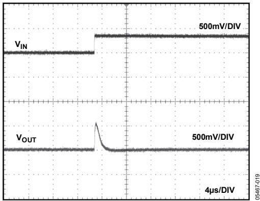
Figure 27. ADR366 Line Transient Response (Increasing), No Capacitors
