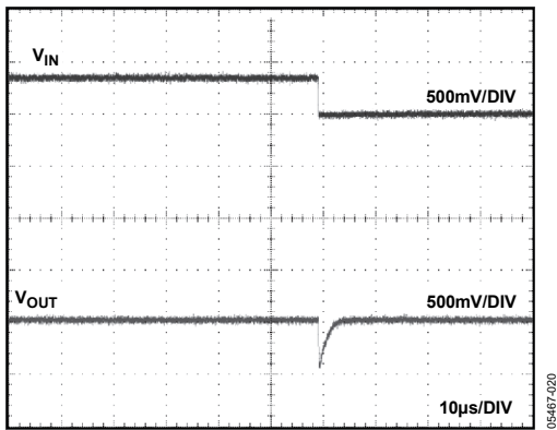
Figure 28. ADR366 Line Transient Response (Decreasing), No Capacitors
