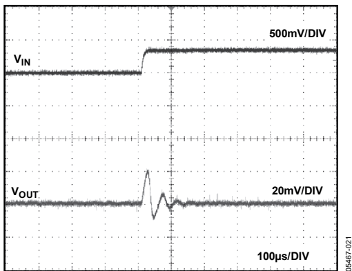
Figure 29. ADR366 Line Transient Response, 0.1 \mu F Input Capacitor
