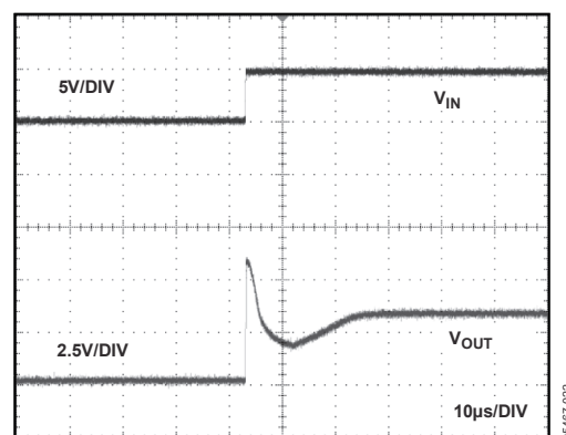
Figure 32. ADR366 Turn On Response Time at 5 V
