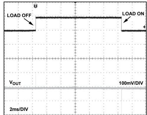
Figure 30. ADR365 Load Transient Response
