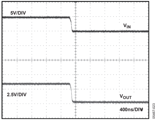
Figure 33. ADR365 Turn Off Response Time at 5 V
