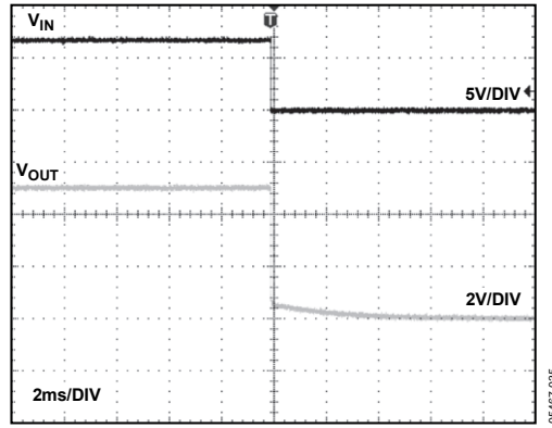
Figure 35. ADR365 Turn Off Response Time, 0.1 \mu F Output Capacitor
