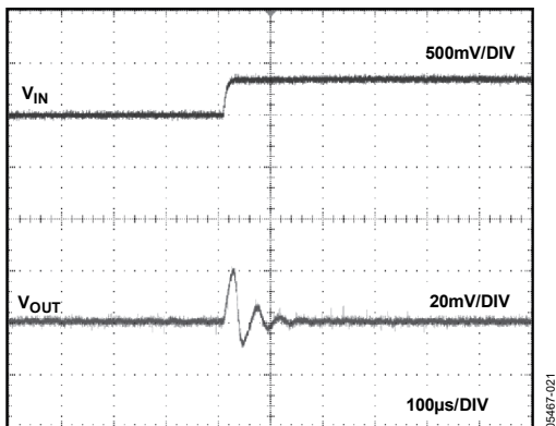
Figure 29. ADR365 Line Transient Response, 0.1 \mu\text{F} Input Capacitor
