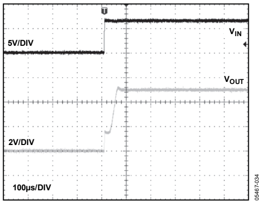
Figure 34. ADR365 Turn On Response Time, 0.1 \mu F Output Capacitor
