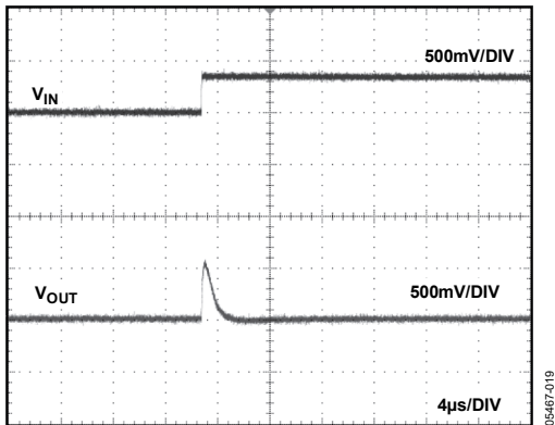
Figure 27. ADR365 Line Transient Response (Increasing), No Capacitors
