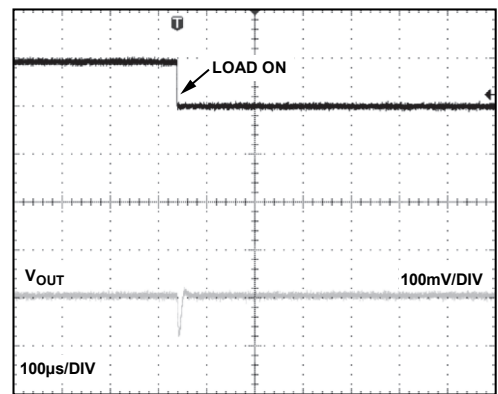
Figure 31. ADR365 Load Transient Response with 0.1 \mu\text{F} Output Capacitor
