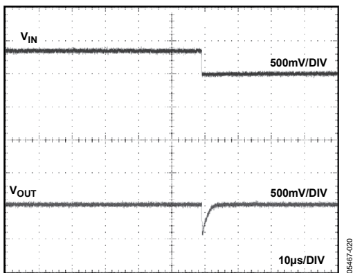
Figure 28. ADR365 Line Transient Response (Decreasing), No Capacitors
