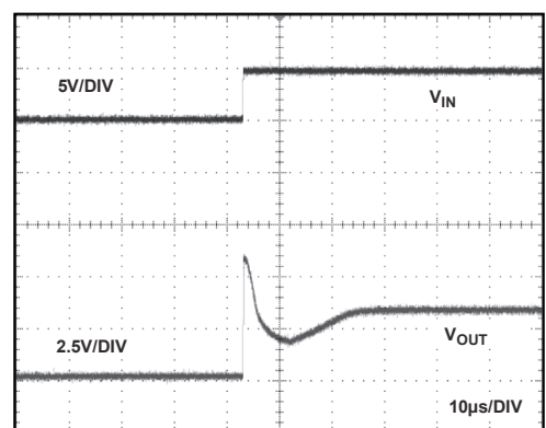
Figure 32. ADR365 Turn On Response Time at 5 V
