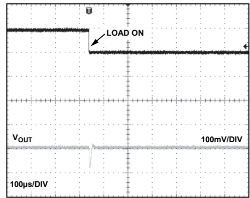
Figure 31. ADR364 Load Transient Response with 0.1 \mu F Output Capacitor
