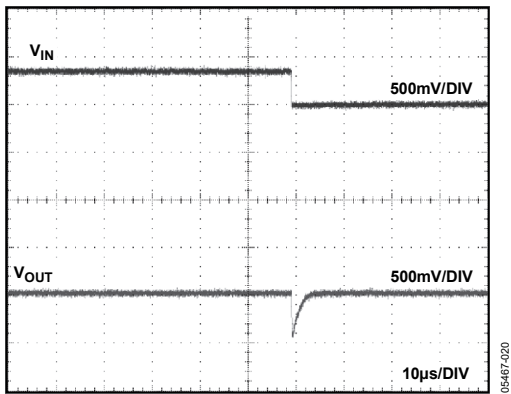
Figure 28. ADR364 Line Transient Response (Decreasing), No Capacitors
