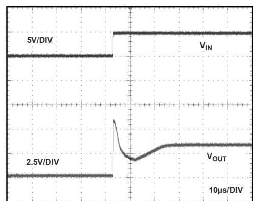
Figure 32. ADR364 Turn On Response Time at 5 V
