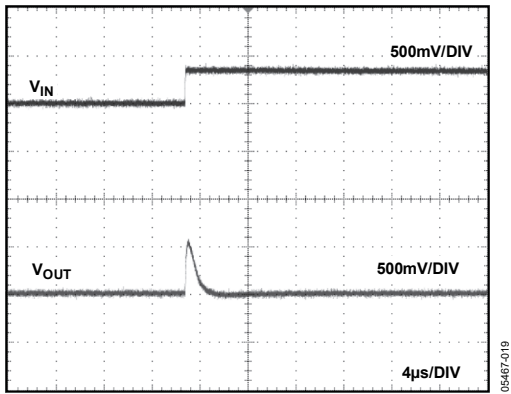
Figure 27. ADR364 Line Transient Response (Increasing), No Capacitors
