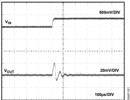
Figure 29. ADR364 Line Transient Response, 0.1 \mu F Input Capacitor
