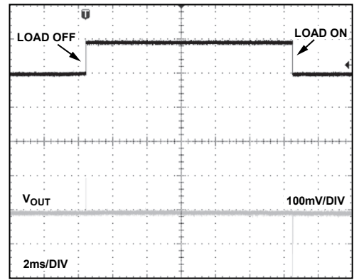
Figure 30. ADR364 Load Transient Response
