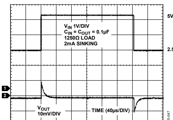
Figure 43. ADR121 Load Transient Response (Sinking)
