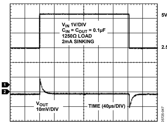
Figure 43. ADR121 Load Transient Response (Sinking)
