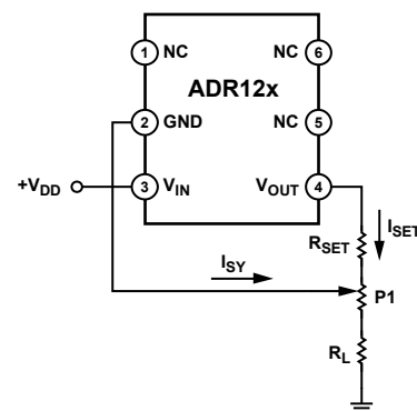
Figure 52. ADR12x Trim Configuration
