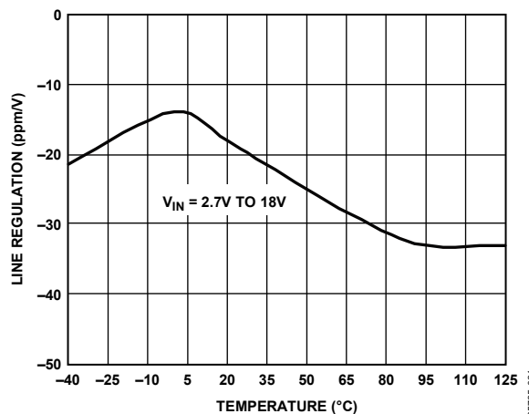
Figure 17. ADR127 Line Regulation vs. Temperature
