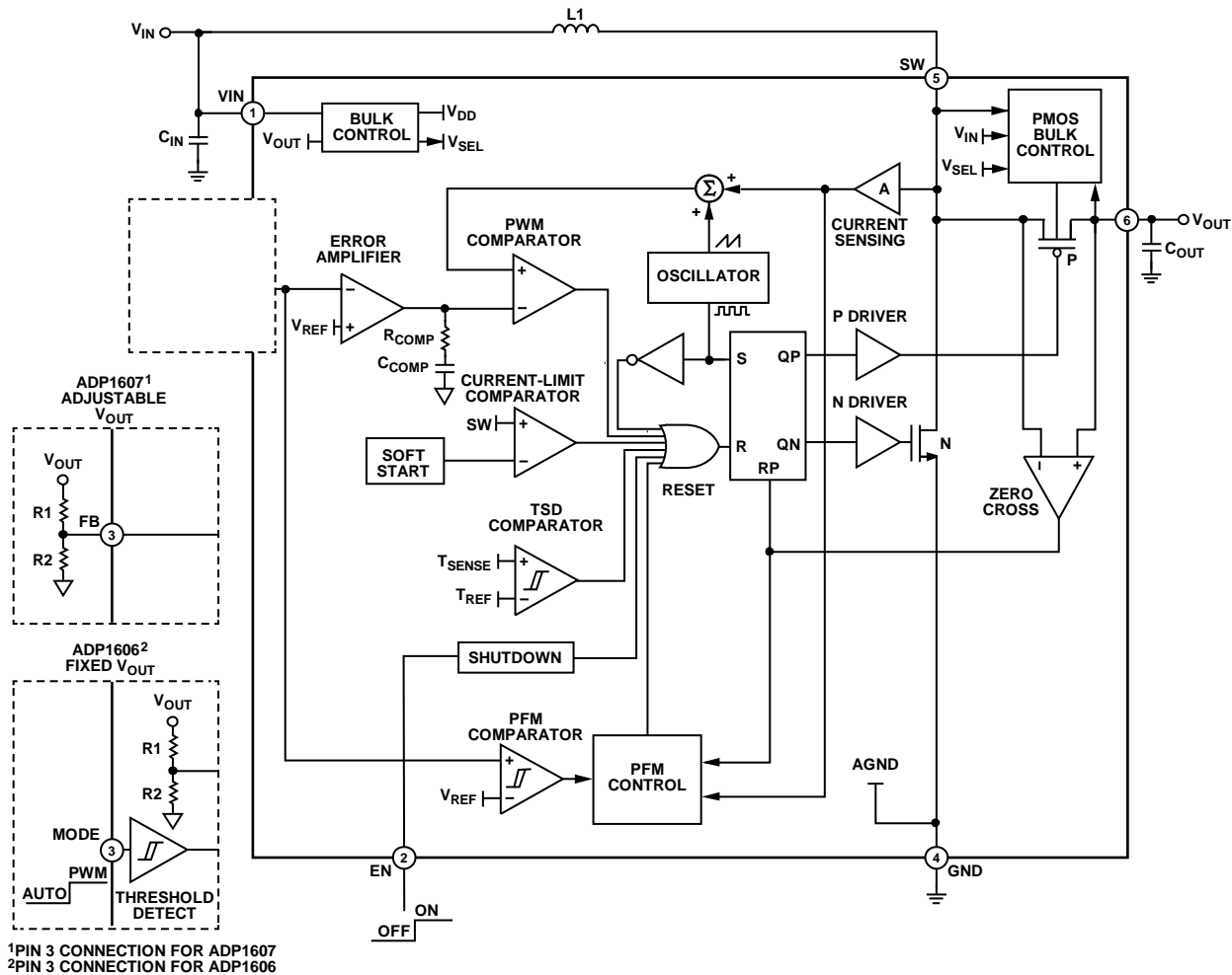
Figure 28. Block Diagram
