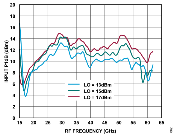
Figure 62. Input P1dB vs. RF Frequency at Various LO Power Levels, TA = 25°C
