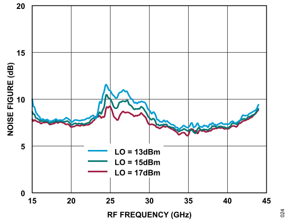
Figure 24. Noise Figure vs. RF Frequency at Various LO Power Levels, TA = 25°C
