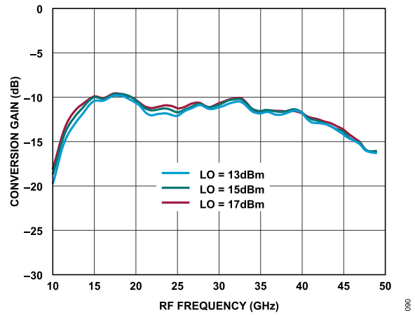
Figure 90. Conversion Gain vs. RF Frequency at Various LO Power Levels, TA = 25°C
