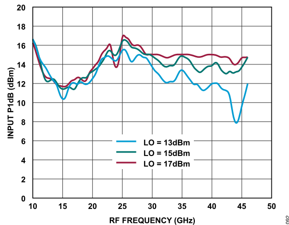
Figure 92. Input P1dB vs. RF Frequency at Various LO Power Levels, TA = 25°C
