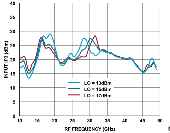
Figure 91. Input IP3 vs. RF Frequency at Various LO Power Levels, TA = 25°C
