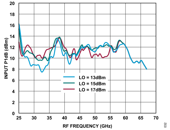
Figure 32. Input P1dB vs. RF Frequency at Various LO Power Levels, TA = 25°C
