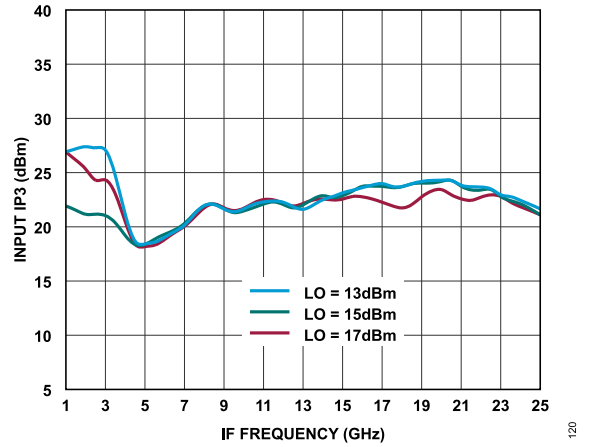
Figure 120. Input IP3 vs. IF Frequency at Various LO Power Levels, T_A = 25^\circ\text{C}
