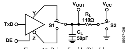
Figure 32. Driver Enable/Disable
