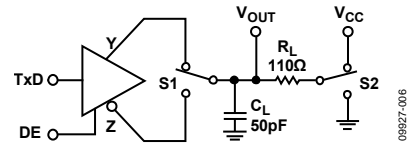
Figure 32. Driver Enable/Disable
