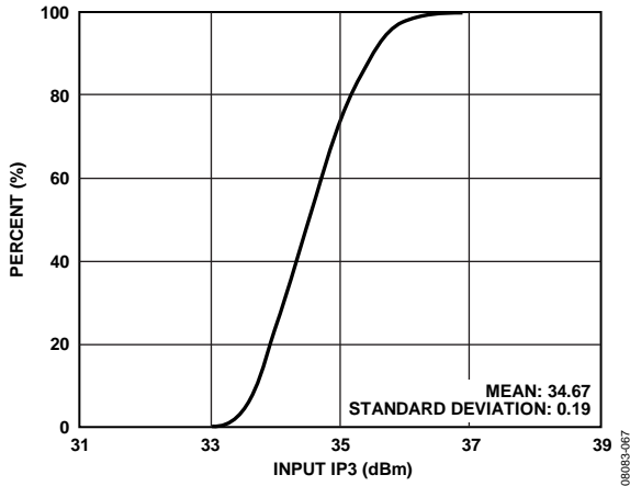
Figure 24. Input IP3 Distribution
