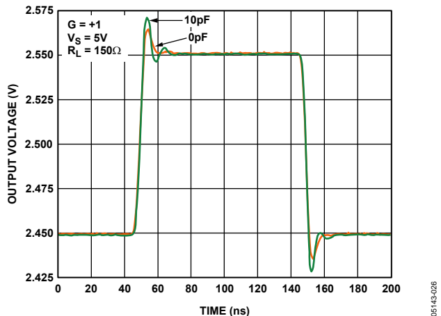
Figure 22. Small-Signal Transient Response for Various Capacitive Loads
