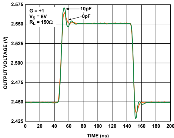
Figure 22. Small-Signal Transient Response for Various Capacitive Loads
