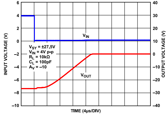
Figure 59. Negative Overload Recovery, V_{SY} = \pm 27.5V
