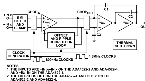
Figure 71. ADA4522-1/ADA4522-2/ADA4522-4 Architecture Block Diagram
