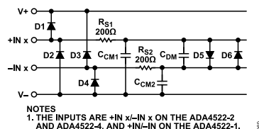
Figure 72. Input EMI Filter and Clamp Circuit
