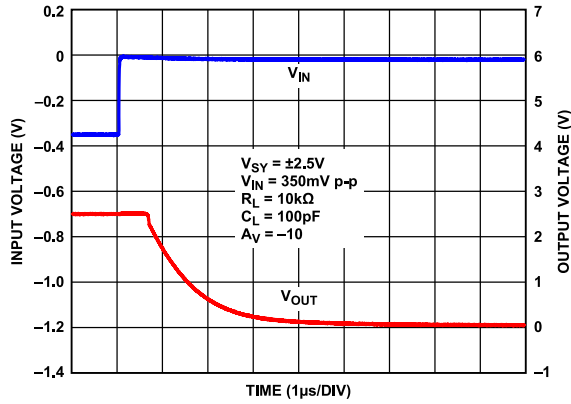
Figure 54. Positive Overload Recovery, V_{SY} = \pm 2.5\text{ V}
