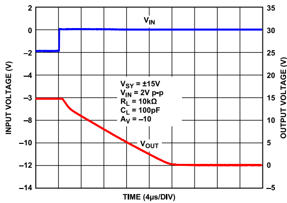
Figure 55. Positive Overload Recovery, V_{SY} = \pm 15\text{ V}
