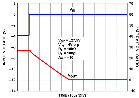
Figure 56. Positive Overload Recovery, V_{SY} = \pm 27.5\text{ V}
