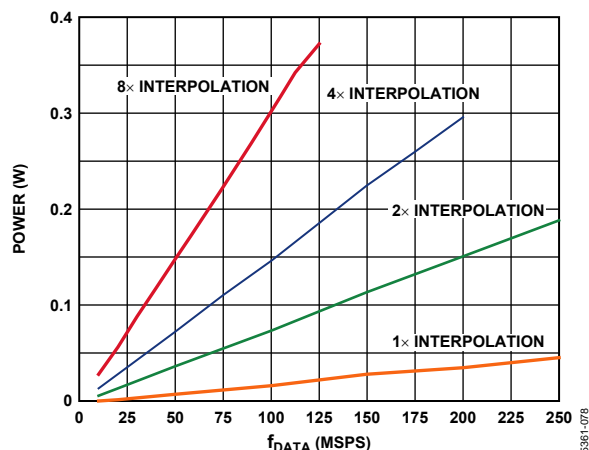
Figure 82. Power Dissipation, Digital 1.8 V Supply, I Data Only, Real Mode, Does Not Include Zero Stuffing
