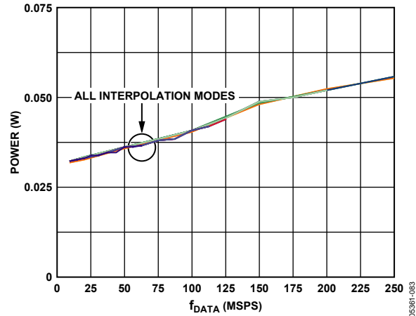
Figure 88. Digital 3.3 V Supply, I and Q Data, Dual DAC Mode
