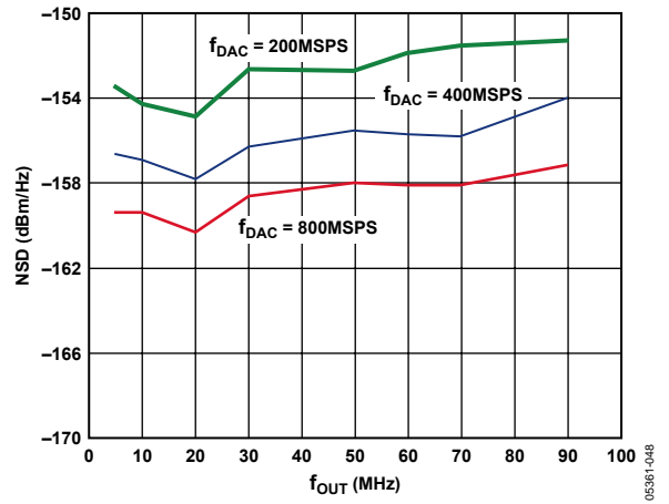
Figure 51. AD9776 Noise Spectral Density vs. f_{DAC} , Single-Tone Input at -6 dBFS, f_{DATA} = 200 MSPS
