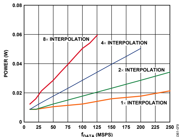
Figure 83. Power Dissipation, Clock 1.8 V Supply, I Data Only, Real Mode, Includes Modulation Modes, Does Not Include Zero Stuffing
