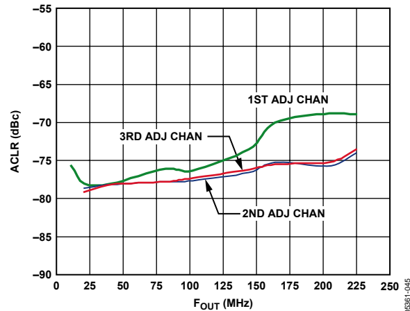
Figure 48. AD9776 ACLR, f_{DATA} = 122.88 \text{ MSPS} , 4x Interpolation, f_{DAC}/4 Modulation
