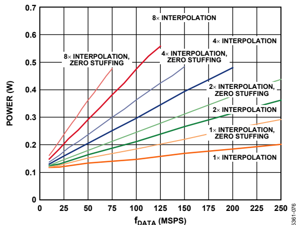
Figure 81. Total Power Dissipation, I Data Only, Real Mode
