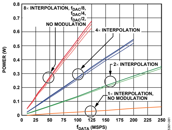
Figure 86. Power Dissipation, Digital 1.8 V Supply, I and Q Data, Dual DAC Mode, Does Not Include Zero Stuffing
