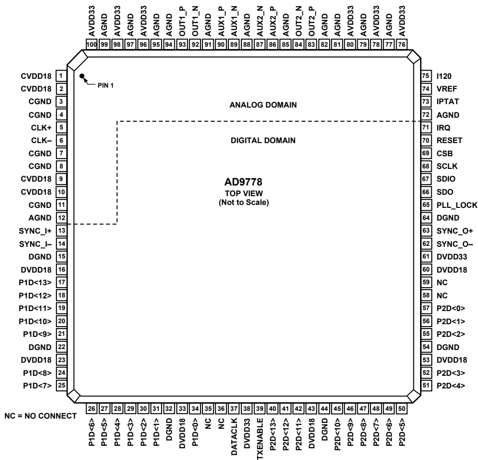
Figure 4. AD9776 Pin Configuration
