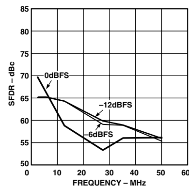
Figure 26. SFDR vs. f_{OUT} @ 125 MSPS
