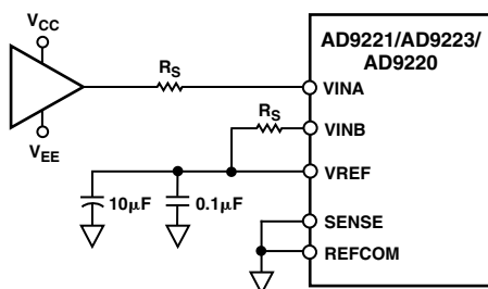
Figure 7. Series Resistor Isolates Switched-Capacitor SHA Input from Op Amp. Matching Resistors Improve SNR Performance
