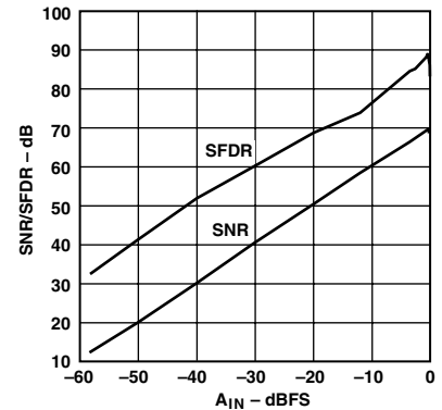
TPC 9. SNR/SFDR vs. A_{IN} (Input Amplitude) ( f_{IN} = 500 \text{ kHz} , Input Span = 2 V p-p, V_{CM} = 2.5 \text{ V} )
