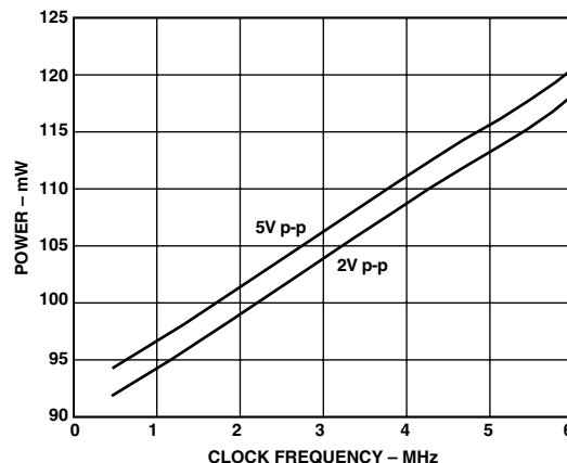
Figure 29b. AD9223 Power Consumption vs. Clock Frequency
