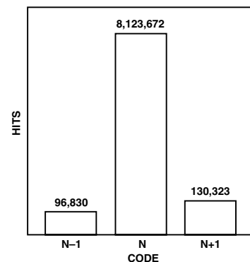
TPC 12. "Grounded-Input" Histogram (Input Span = 2 V p-p)
