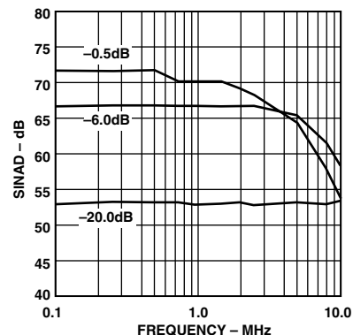
TPC 15. SINAD vs. Input Frequency (Input Span = 5.0 V p-p, V_{CM} = 2.5\text{ V} )
