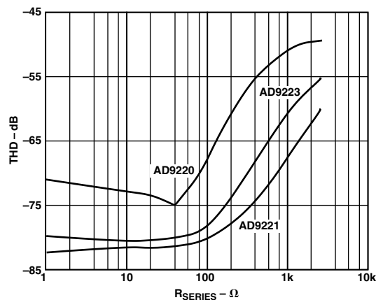
Figure 8. THD vs. R_{SERIES} ( f_{IN} = f_S/2 , A_{IN} = -0.5 dB, Input Span = 2 V p-p, V_{CM} = 2.5 V)
