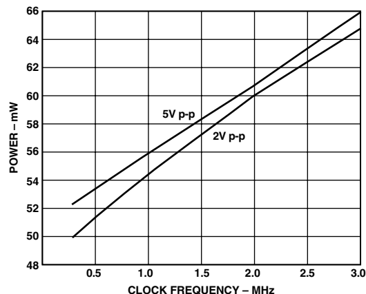
Figure 29a. AD9221 Power Consumption vs. Clock Frequency
