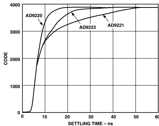
Figure 3. Settling Time
