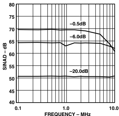
TPC 13. SINAD vs. Input Frequency (Input Span = 2.0 V p-p, V_{CM} = 2.5\text{ V} )
