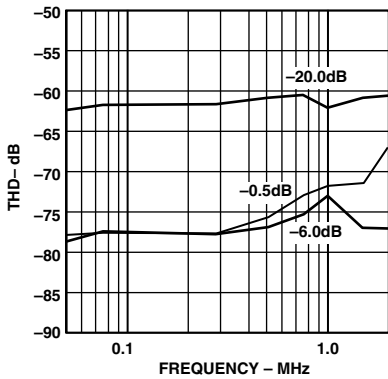
TPC 7. THD vs. Input Frequency (Input Span = 5.0 V p-p, V_{CM} = 2.5 \text{ V} )
