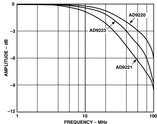
Figure 2. Full-Power Bandwidth
