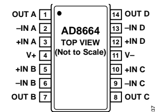
Figure 6. AD8664, 14-Lead TSSOP (RU-14)
