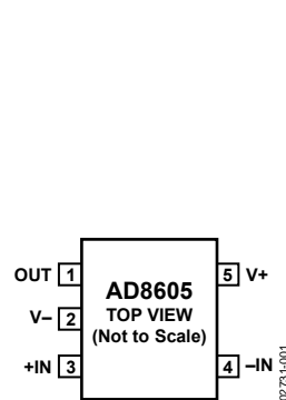
Figure 1. 5-Lead SOT-23 (RJ Suffix)
