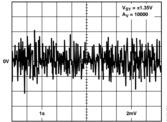
Figure 38. 0.1 Hz to 10 Hz Noise at 2.7 V
