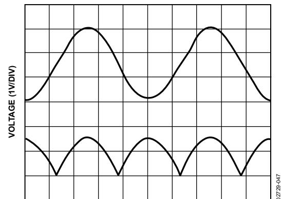
TIME (1ms/DIV)
