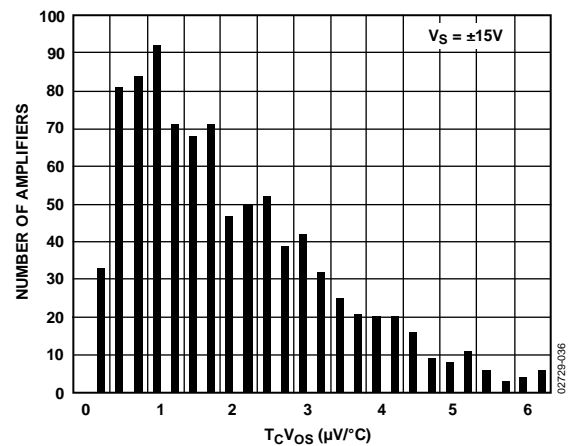
Figure 36. AD8512 T_C V_{OS} Distribution
