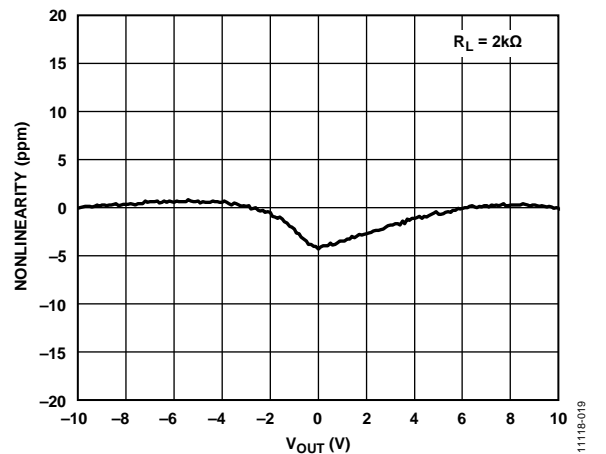
Figure 22. Gain Nonlinearity
