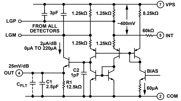
Figure 31. Simplified Output Interface
