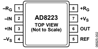
Figure 2. Pin Configuration
