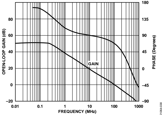
Figure 35. Open-Loop Gain and Phase vs. Frequency
