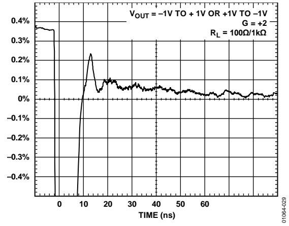
Figure 27. Settling Time
