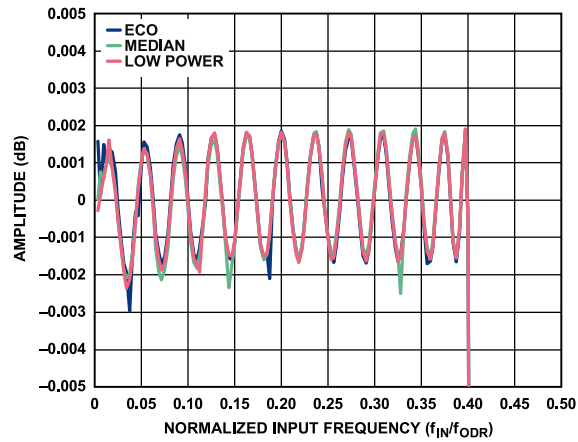
Figure 59. Wideband Filter Ripple
