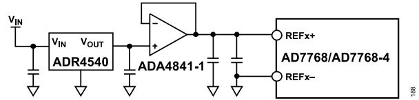
Figure 88. Typical Reference Input Configuration Diagram
