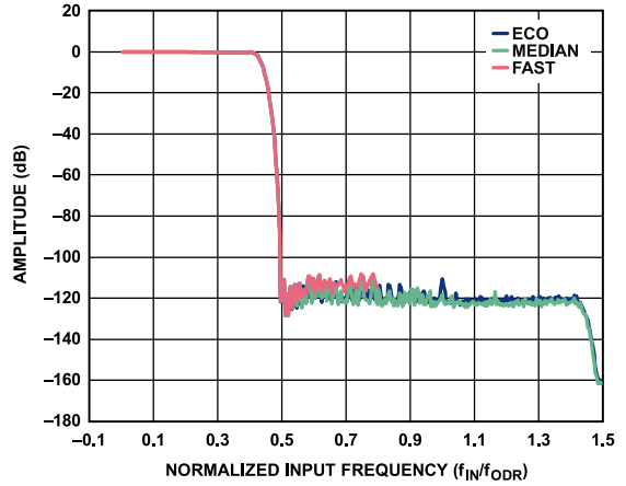
Figure 57. Amplitude vs. Normalized Input Frequency ( f_{IN}/f_{ODR} ), Wideband Filter Profile
