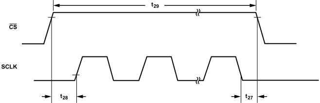
Figure 9. SCLK Enable and Disable Timing Diagram
