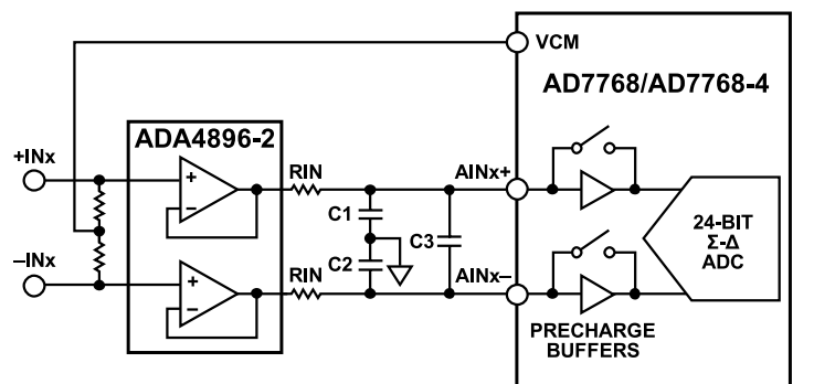
Figure 87. Typical Input Structure for an RC Network
