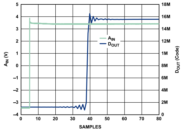
Figure 58. Step Response, Wideband Filter
