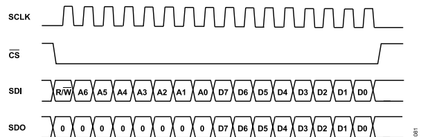
Figure 80. Write/Read Command
