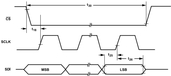
Figure 8. SPI Serial Write Timing Diagram
