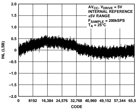
Figure 16. AD7606 Typical INL, \pm 5 V Range
