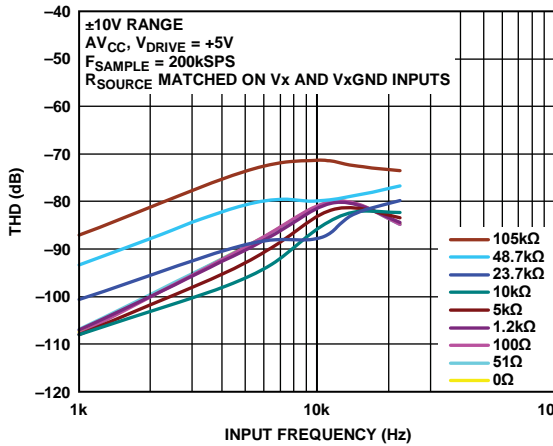
Figure 24. THD vs. Input Frequency for Various Source Impedances, ±10 V Range
