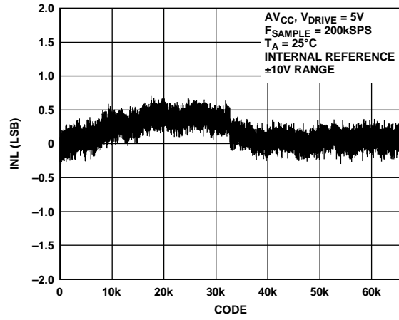
Figure 14. AD7606 Typical INL, \pm 10 V Range
