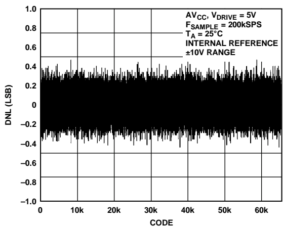
Figure 15. AD7606 Typical DNL, \pm 10 V Range
