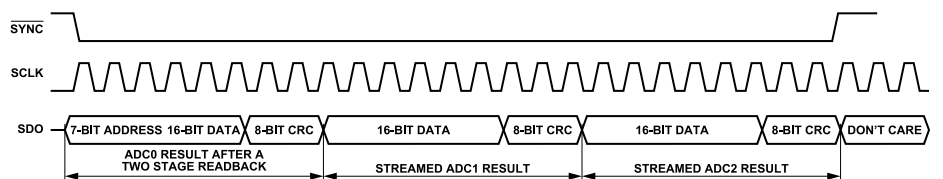
Figure 60. Burst Read Mode SDO Contents
