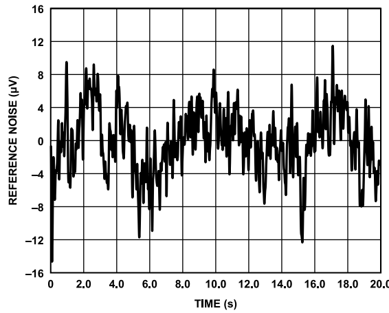
Figure 18. Peak-to-Peak Noise (0.1 Hz to 10 Hz Bandwidth)
