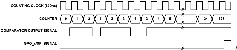
Figure 43. Digital Input Debounce Mode 0 Timing Example
