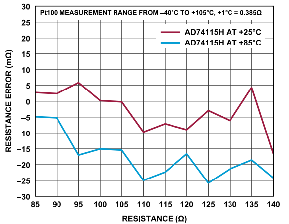
Figure 15. 3-Wire RTD Measurement Error
