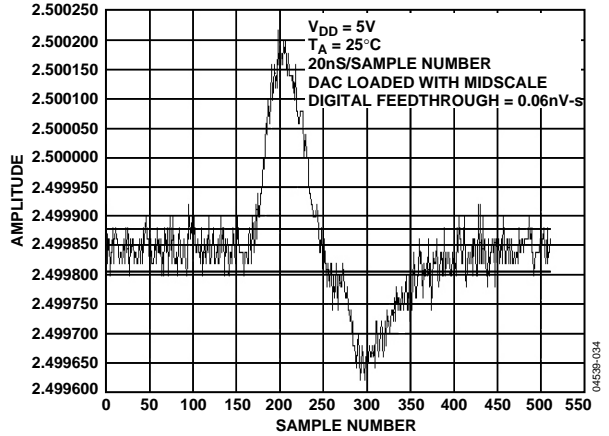
Figure 34. Digital Feedthrough
