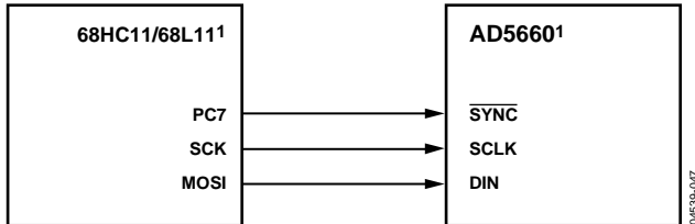
Figure 47. AD5660-to-68HC11/68L11 Interface
