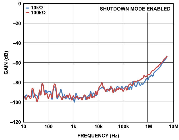
Figure 29. Shutdown Isolation vs. Frequency
