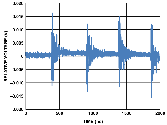
Figure 28. Digital Feedthrough
