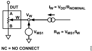
Figure 33. Wiper Resistance
