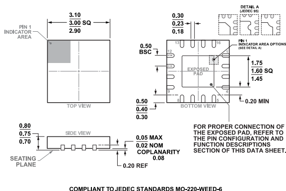
Figure 41. 16-Lead Lead Frame Chip Scale Package [LFCSP] 3 mm x 3 mm Body and 0.75 mm Package Height (CP-16-22) Dimensions shown in millimeter
