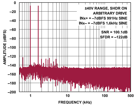
Figure 25. FFT, 1 MSPS, f_{INx+} = 991 Hz, f_{INx-} = 1.6 kHz, ±40 V Range
