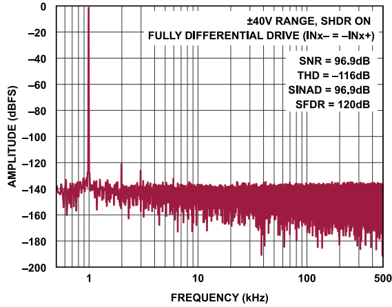
Figure 21. FFT, 1 MSPS, f_{IN} = 1 kHz, ±40 V Range
