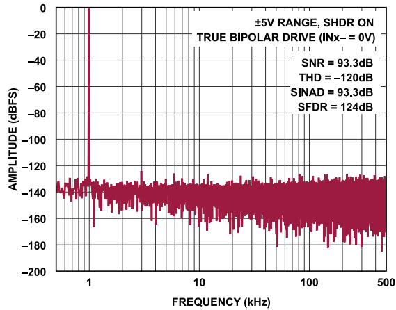
Figure 22. FFT, 1 MSPS, f_{IN} = 1 kHz, ±5 V Range
