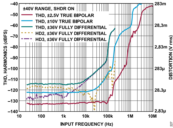
Figure 27. THD, Harmonics vs. Input Frequency
