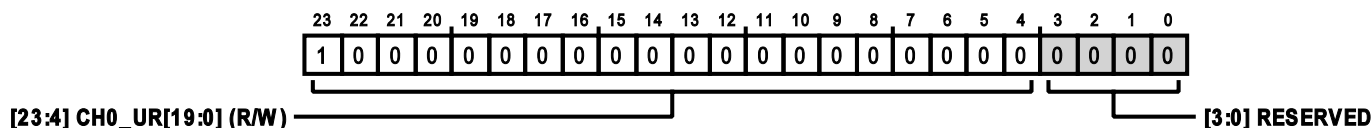
Figure 105. Address: 0x35 to Address 0x37, Reset: 0x80000, Name: CH0_UR
