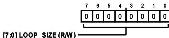
Figure 86. Address: 0x0E, Reset: 0x00, Name: LOOP_CONFIG_A
