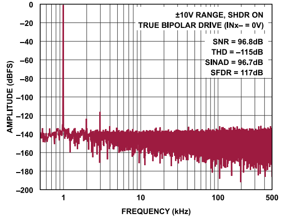
Figure 24. FFT, 1 MSPS, f_{IN} = 1 kHz, ±10 V Range
