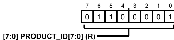
Figure 79. Address: 0x04, Reset: 0x61, Name: PRODUCT_ID_L
