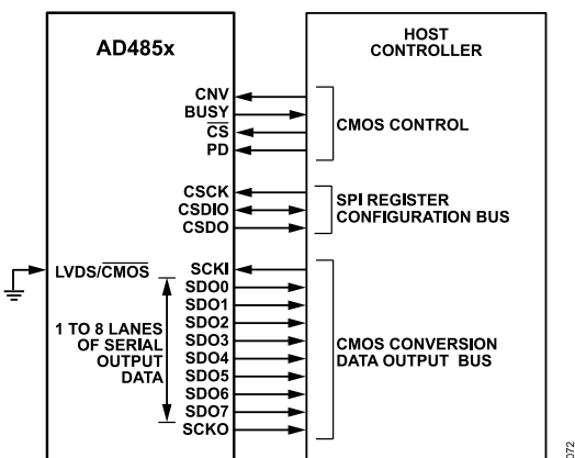
Figure 65. CMOS Conversion Data Output Mode for the AD4857
