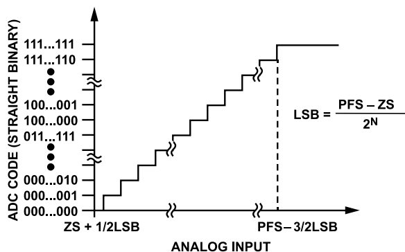
Figure 50. AD4857 Ideal Unipolar Input Transfer Function, N = 16 Bits
