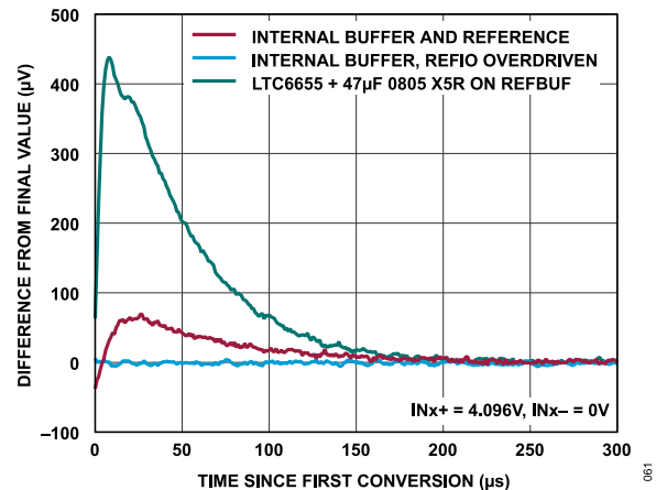
Figure 60. Burst Conversion Response of the AD4857, f_S = 1 MSPS
