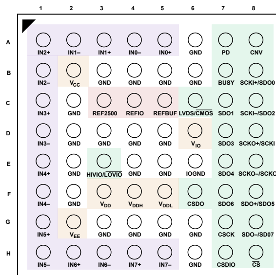
AD4857 TOP VIEW (Not to Scale)
